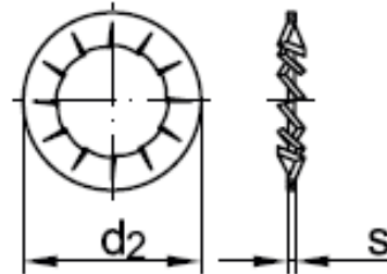
Form I = innengezahnt
